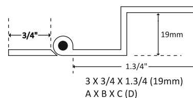
“L” Hinges
