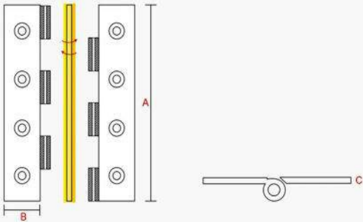
BRASS BUTT HINGES WITH CENTRE PIN LOCK
