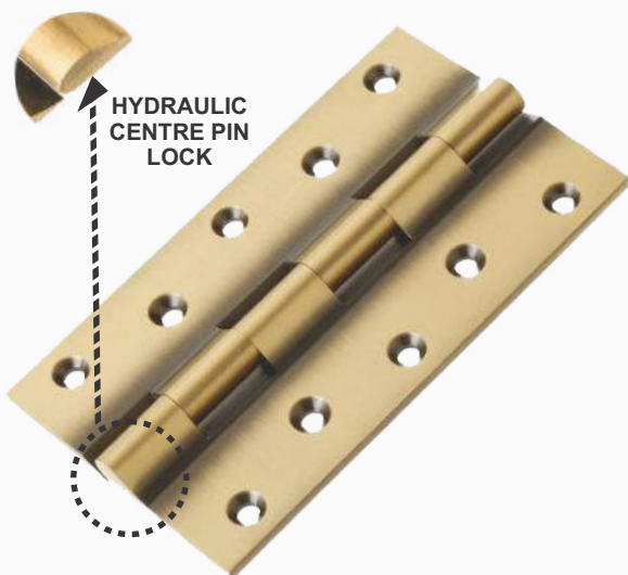
RAILWAY HINGES WITH HYDRAULIC CENTRE PIN LOCK
