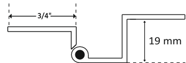
Smooth "W" Hinges
