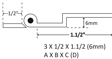
“L” Hinges
