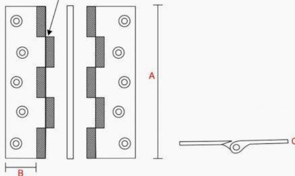
RAILWAY HINGES WITH SS 304 WASHER
