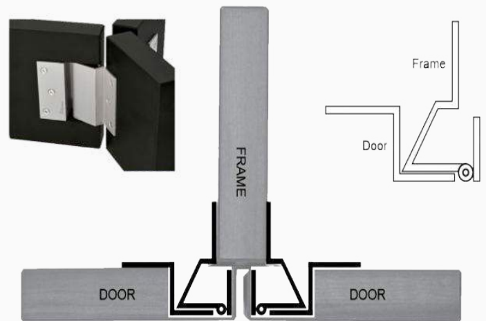
HALF OVERLAY
