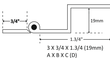
Smooth "L" Hinges
