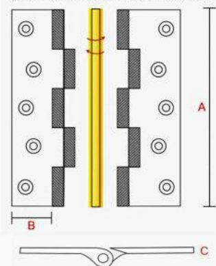
COMMERCIAL RAILWAY HINGES WITH CENTRE PIN LOCK
