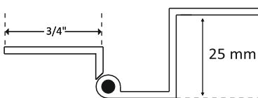
Smooth "W" Hinges
