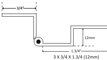
Smooth "W" Hinges
